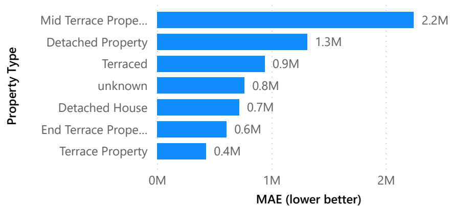
Prediction Error by Property Type (MAE)
