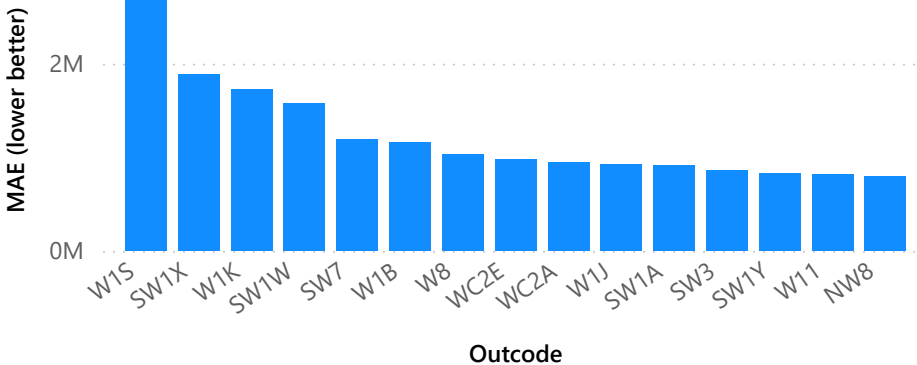
Top 15 Highest-Error Locations
